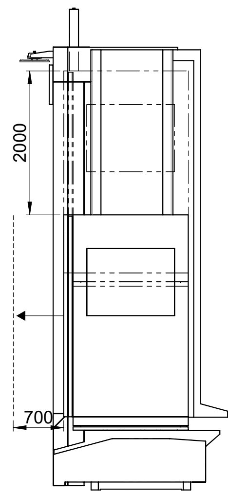
CORSE PEDANA OPERATORE OPERATOR PLATFORM'S STROKES
